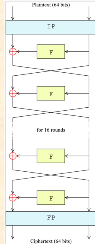
Figure 1— The overall Feistel structure of DES
